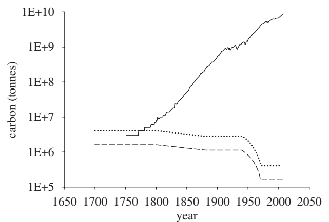
Figure 1. Carbon export from, and input to, the atmosphere from 1700 to 2005 including carbon emissions from fossil fuel burning, carbon export stimulated by iron defecated by Southern Ocean sperm whales and carbon respired by Southern Ocean sperm whales. Solid line, carbon from fossil fuels; dotted line, carbon exported; dashed line, carbon respired.
