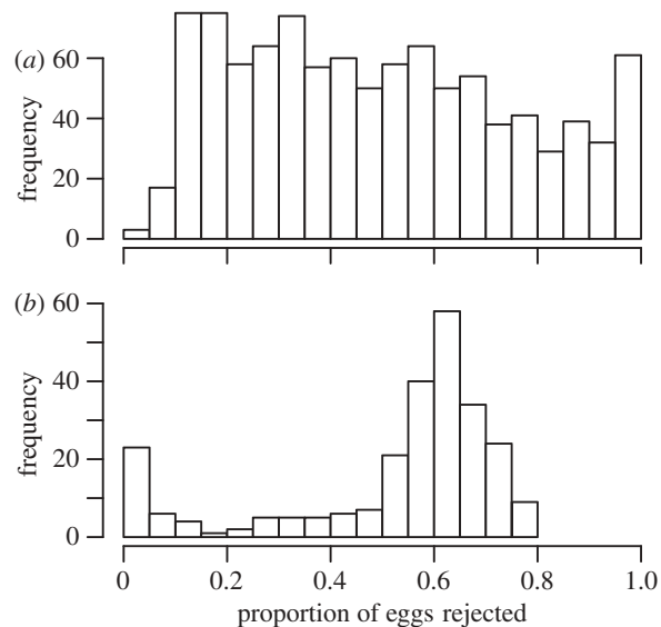
Figure 3. Rejection frequency by each host species of real cuckoo finch eggs laid by their respective parasitic genes, based on simulations using logistic models of egg discrimination experiments (see §2). Total frequencies add up to in (a) 999, tawny-flanked prinias, but in (b) 250, red-faced cisticolas (see §2).
