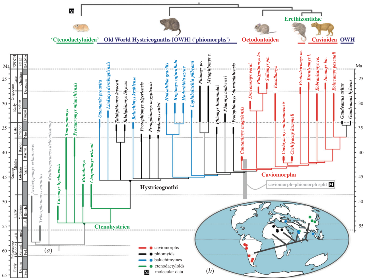
Figure 3. Phylogeny and dispersal scenario of Palaeogene caviomorph rodents and related taxa. (a) Phylogeny of Contamana rodents among Palaeogene ctenohystricans (Ctenohystrica), hystricognaths (Hystricognathi) and caviomorphs (Caviomorpha). Strict consensus cladogram obtained with a maximum-parsimony PAUP (phylogenetic analysis using parsimony) heuristic search (see the electronic supplementary material). The consistency (CI), retention (RI) and homoplasy (HI) indices of the 13 shortest trees (859 steps) are 0.33, 0.63 and 0.68, respectively. Branch support of the concerned nodes (Bremer indices) appears in the electronic supplementary material, figure S2a. Contamana rodents included in this analysis (bold type) are stem caviomorphs (i.e. not referable to Octodontoidea, Erethizontidae or Caviioidea). cf. Eoespina sp. (not included, two teeth) is interpreted as a stem octodontoid. Eobranisamys sp. (four teeth) might be connected to the Eobranisamys romeropitmanae branch (Caviioidea), which suggests a late Middle Eocene age for the common ancestor of cavioids. Sister-group relationships between Gaudeamus (advanced phiomorph; Old World Hystricognath, OWH) and Eoincamys (caviomorph) probably document a striking convergent dental evolution [11,14], rather than independent dispersal from South America to Africa. Light-grey shaded bar illustrates molecular estimate ranges for the caviomorph–phiomorph split (CPS; 45.4 \pm 4.1 Ma [9]), thus located behind the morphologically supported CPS node (grey triangle). On top, dark-grey tree sketches phylogenetic relationships among living ctenohystricans as supported by molecular data [9]. Barran., Barrancon; Barton., Bartonian; Itab., Itaboraian; Mus., Mustersan; Pel., Peligran; Priabon., Priabonian; Rioch., Riochican; SALMA, South American Land Mammal Age; Seland., Selandian; Thanet., Thanetian; Tingui., Tinguirirican; Species name abbreviations: bo. , bolivianus ; br. , brachyodon ; l. , luribayensis ; m. , medianus ; pa. , pascualii ; pr. , paraphiomyoides ; ro. , romeropitmanae ; s. , schaubi . Rodent drawings by M. J. Orliac. See the electronic supplementary material for further details. (b) Palaeogeographic world map at 40 Ma and privileged phylogeographic sketch of Palaeogene hystricognath rodents, as inferred by both the consensus tree shown in (a) and the geographical range of concerned taxa (coloured circles; same colour codes as in (a)).
