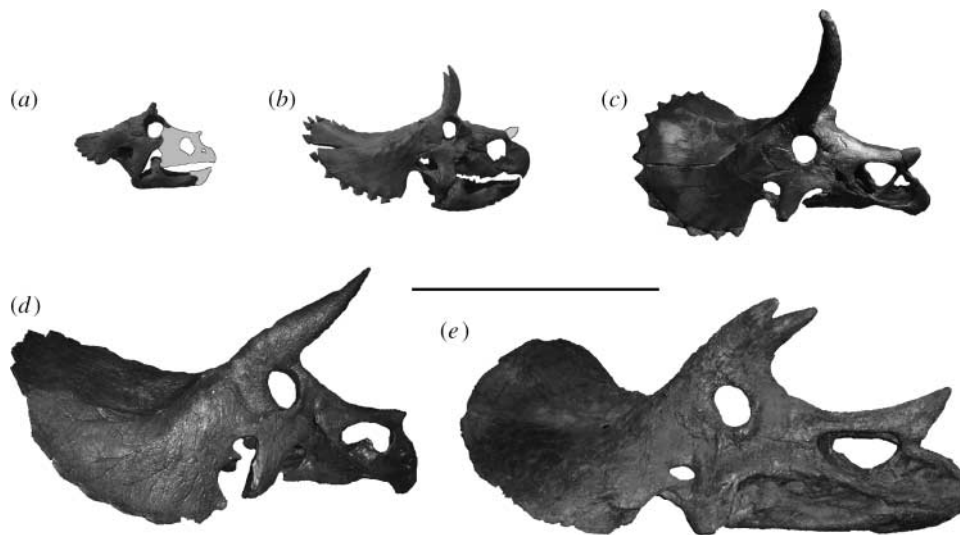
Figure 1. Five examples of the four cranial ontogenetic growth stages in Triceratops skulls in right lateral view. Skull length is given in parentheses. (a) UCM 154452, baby skull (38 cm); (b) MOR 1199, small juvenile skull (87 cm); (c) MOR 1110, large juvenile skull (135 cm); (d) MOR 1120, subadult skull (165 cm); and (e) MOR 004, adult skull (208 cm). Reconstructed area of (a) UCM 154452 and the epinasal in (b) MOR 1199 are drawn in white. Scale bar, 1 m.
