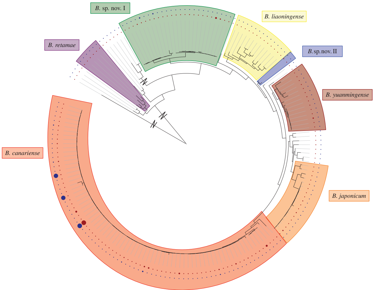
Figure 1. Reconstructed phylogram of CHR haplotypes. Tree reconstructed in PHML using concatenated dnak , glnII , ITS and recA loci. Zigzags indicate long branches shortened for visibility. Species-like clades are indicated in shaded portions. The size of the circles on the inner and our perimeter indicate the relative abundance and spatial range, respectively, of each CHR haplotype. (Online version in colour.)
