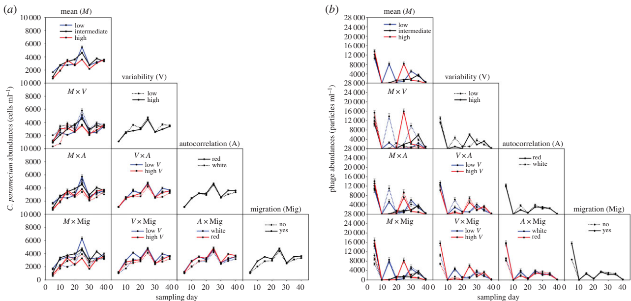
Figure 2. (a) Chilomonas paramecium flagellate and (b) phage Phi2 abundances in different experimental treatments. The main effects of experimental factors are depicted on the diagonal, and two-way interactions between different factors below the diagonal. Line colours in interaction panels depict 'column' factors, and solid and dashed lines the effect of 'row' factor. All lines show \pm 1 s.e.m.
