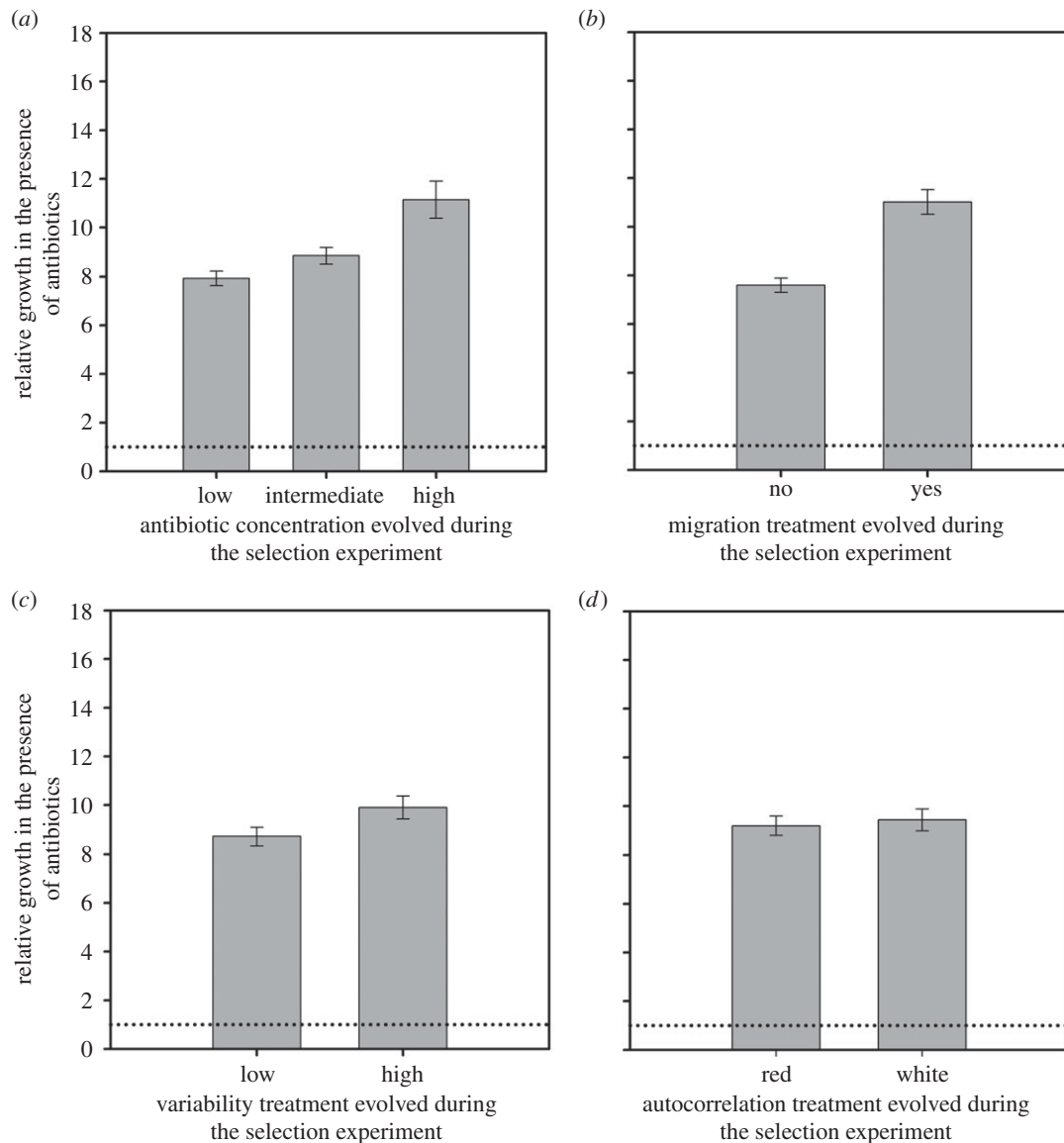
Figure 3. Bacterial adaptation to antibiotics. The effect of mean antibiotic (a) concentration, (b) migration, (c) variability and (d) autocorrelation structure for the fitness of evolved bacteria relative to ancestral bacterium. All bars show \pm 1 s.e.m. These assays were performed at high antibiotic concentration.
