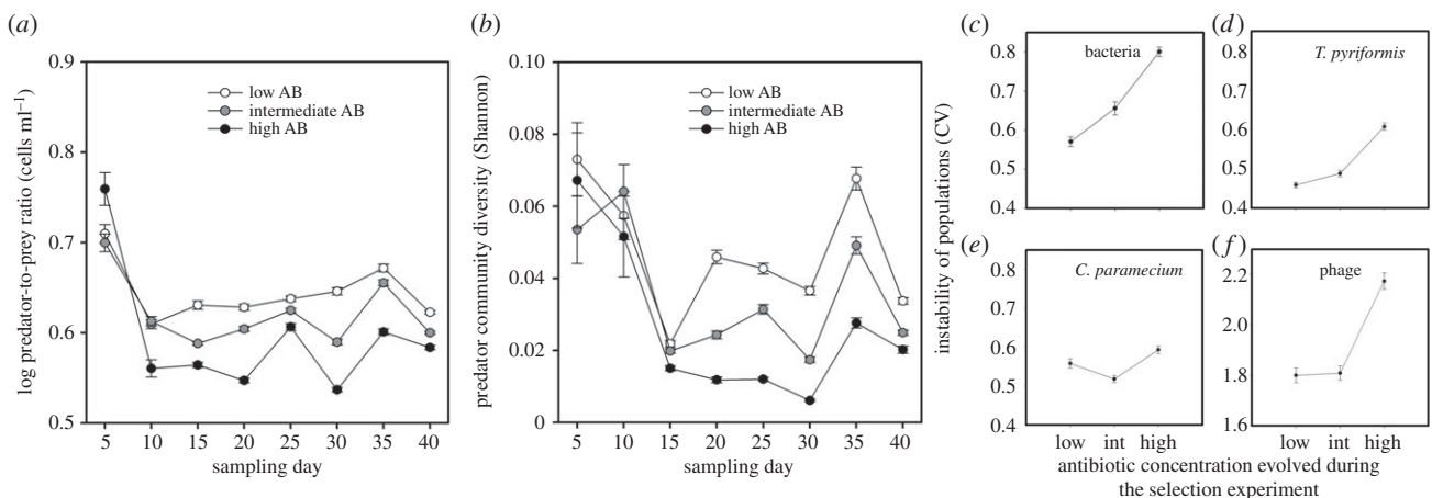
Figure 5. Differences in ecological properties of communities. (a) Predator-to-prey abundance ratio, (b) predator community diversity (alpha diversity, Shannon index) and (c–f) instability of (c) bacterial, (d) T. pyriformis , (e) C. paramecium and (f) phage populations evolved in different antibiotic environment during the selection experiment. AB denotes for antibiotic concentration in panels (a,b) and all bars show \pm 1 s.e.m.
