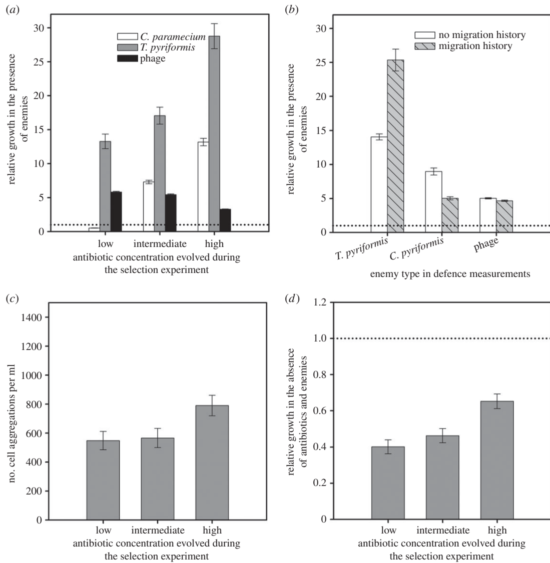
Figure 4. Bacterial adaptation to enemies. (a) Defence evolution against different enemies for bacteria evolved in different antibiotic environments during the selection experiment. (b) Defence evolution against different enemies for bacteria evolved in the absence and presence of migration during the selection experiment. (c) Bacterial cell aggregate formation evolution for bacteria evolved in different antibiotic environments during the selection experiment. (d) Pleiotropic growth cost measured in the absence of enemies and antibiotics for bacteria evolved in different antibiotic environments during the selection experiment. All bars show \pm 1 s.e.m. In (a,b,d), quantities are relative to the ancestral strain.
