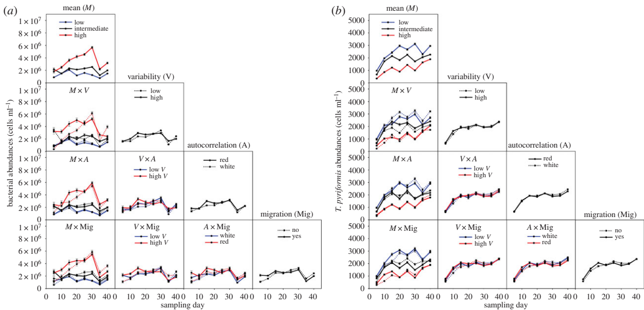
Figure 1. (a) Bacterial and (b) T. pyriformis ciliate abundances in different experimental treatments. The main effects of experimental factors are depicted on the diagonal, and two-way interactions between different factors below the diagonal. Line colours in interaction panels depict 'column' factors, and solid and dashed lines the effect of 'row' factor. All lines show \pm 1 s.e.m.
