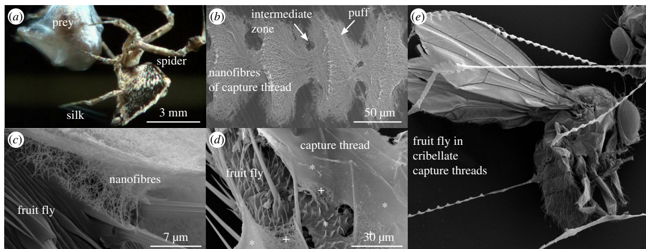
Figure 1. Cribellate spiders capturing prey. (a) U. plumipes (hanging upright) wrapping prey after capturing it in its horizontal orb web. (b) Cribellate capture thread of U. plumipes adhered to a metal surface. The adhesive nanofibres are organized in regularly spaced puffs and intermediate zones. (c) Single nanofibres adhering to prey ( D. melanogaster ). (d) When in contact with D. melanogaster , cribellate threads show areas where single nanofibres (+) are no longer discernible individually (*). (e) Overview of D. melanogaster covered in capture threads of U. plumipes . (b–e) SEM images. (c–e) Provided by H. Adamova. (Online version in colour.)
