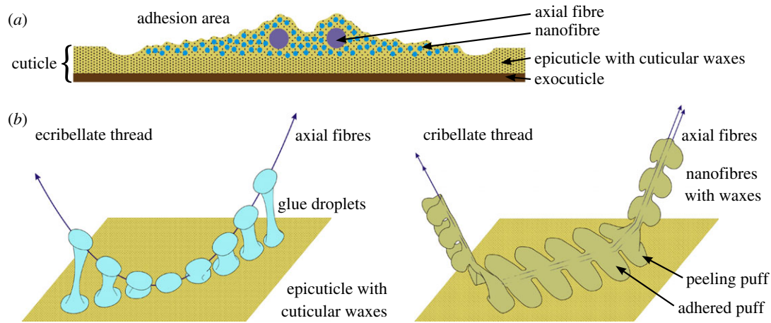
Figure 3. Model of adhesive mechanism of cribellate capture threads. (a) Cross-section of an adhered cribellate thread, showing the nanofibres and the axial fibres embedded in the epicuticular waxes of the prey's cuticle. (b) Comparison of the adhesion mechanism of ecribellate and cribellate threads illustrates differences in their peeling behaviour due to employment of different adhesives. For detaching from a surface, single droplets of viscous glue (ecribellate thread) stretch between prey and capture thread, distributing the applied traction more equally between the points of attachment. By contrast, the single puffs of the cribellate capture thread peel off individually one after another. (Online version in colour.)
