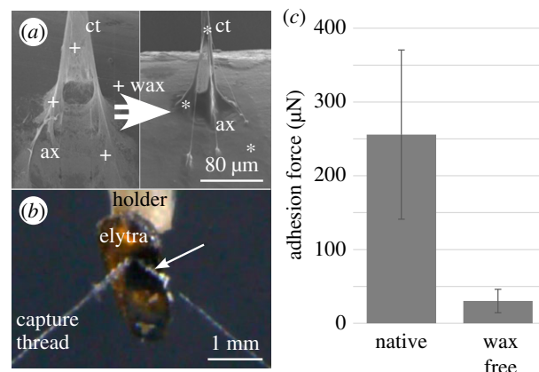
Figure 2. Epicutular waxes enhance adhesion between cribellate capture thread and prey. (a) A cribellate thread (ct) adhered to an untreated metal surface (left panel) shows individual nanofibres (+). Previous coating with epicutular waxes of cowpea weevils, C. maculatus , however, led to a 'fusion' of nanofibres into a homogeneous sheet-like structure (*) (right). Note that in both cases, the axial fibres (ax) are partly separated from the cribellate fibres. SEM image. (b) When pulling a native elytron out of a cribellate capture thread, the separation proceeds by single puffs peeling off individually (arrow; see electronic supplementary material, movie S2). (c) Removal of waxes from the elytra led to a significant decrease in the adhesive force (two-tailed t -test: \alpha = 0.05 ; p = 1.2 \times 10^{-6} ). (Online version in colour.)
