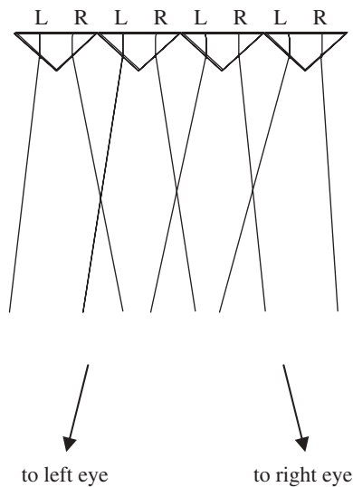
Figure 7. Schema for partitioning a monitor screen into alternate narrow vertical strips containing image segments directed to the left and right eyes, respectively, by suitably deviating their optical paths. Screen and eye positioning are critical.
